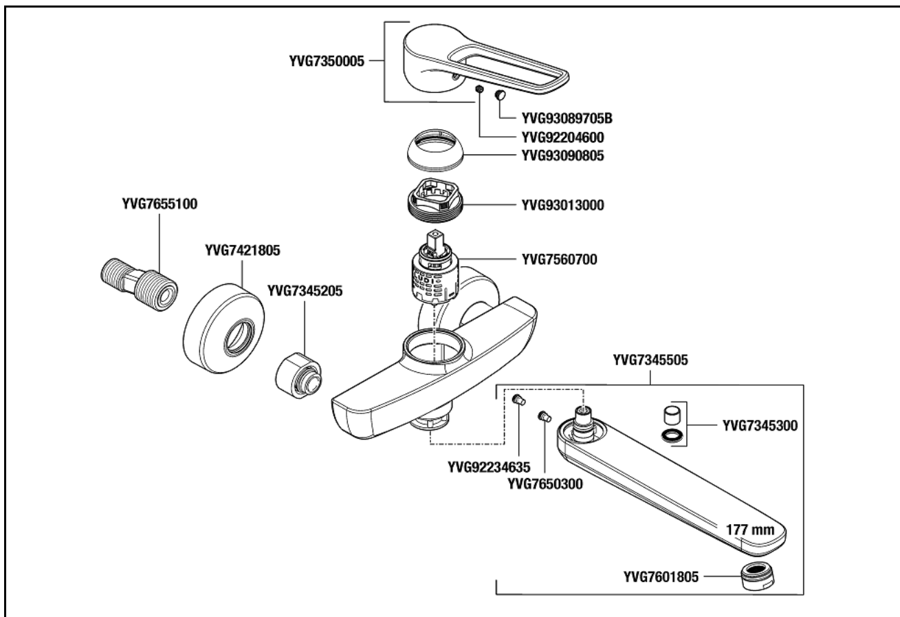
DEPOHWB240 Einhand-Wandbatterie derby plus m. Hebel offen Ausl. 240mm verchromt VIGOUR Wall mounted mixer derby plus w. lever open spout projection 240mm ch. VIGOUR
